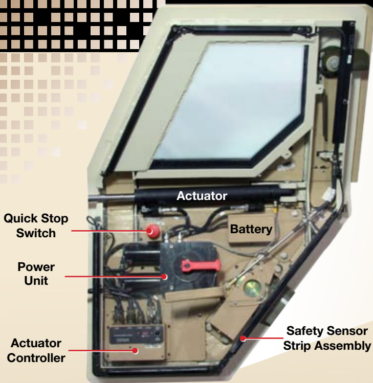
Powered Door System shown using hydraulic actuation
