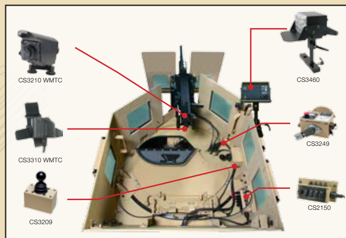
Typical accessories on a M114 with O-GPK
