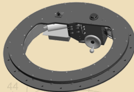
CS6400 Motorized Armored Personnel Carrier Turret (APCT)
