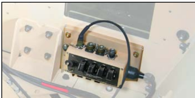
Auxiliary Power Module mounted inside O-GPK
